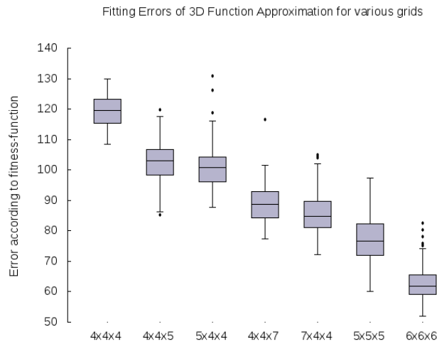
Figure 5.7: The fitting error for the various grids we examined. Note that the number of control–points is a product of the resolution, so X \times 4 \times 4 and 4 \times 4 \times X have the same number of control–points.
